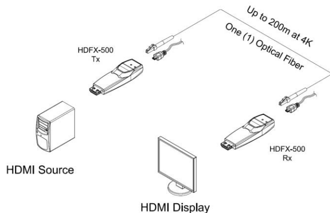
Figure 1 – Overall Connection of HDFX-500-TR
